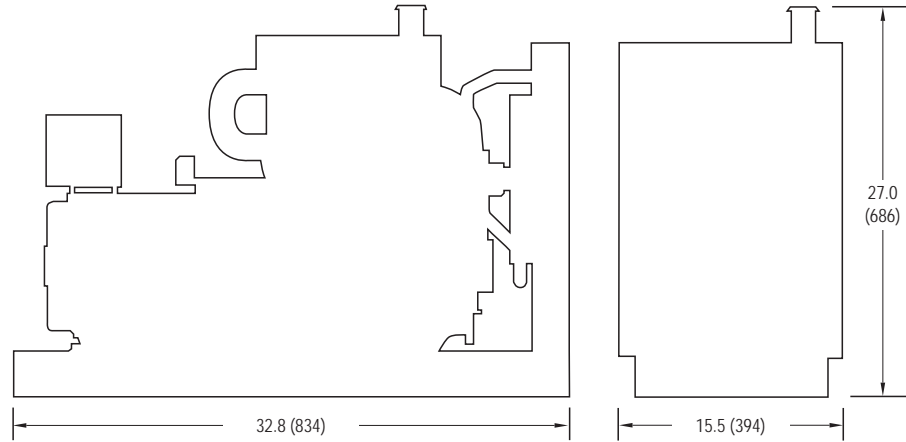
NL673L3 Overall Dimensions L x W x H: 32.8 x 15.5 x 27.0 inch (834 x 394 x 686 mm)
